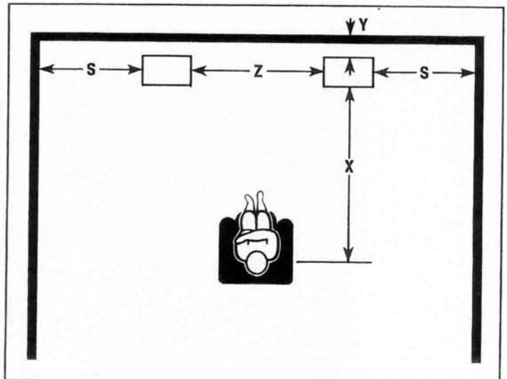
FIGURE 3. Speaker Placement
