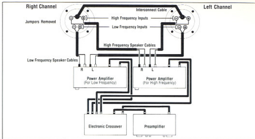
FIGURE 8. Connections for Bi-Amplification using an Electronic Crossover
