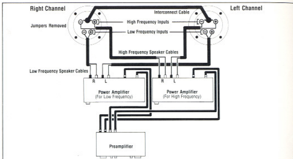
FIGURE 7. Connections for Bi-Amplification
