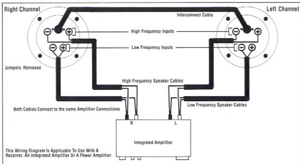
FIGURE 6. Connections for Bi-Wiring
