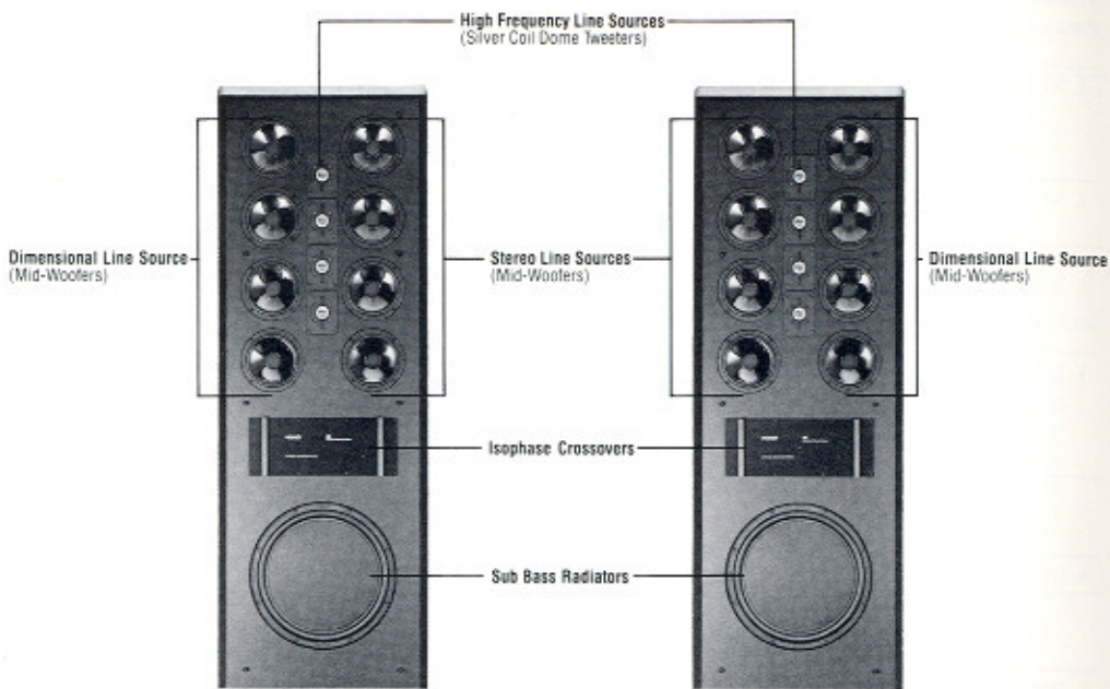
FIGURE 14. Front View of the SDA SRS Loudspeakers with Grilles Removed
